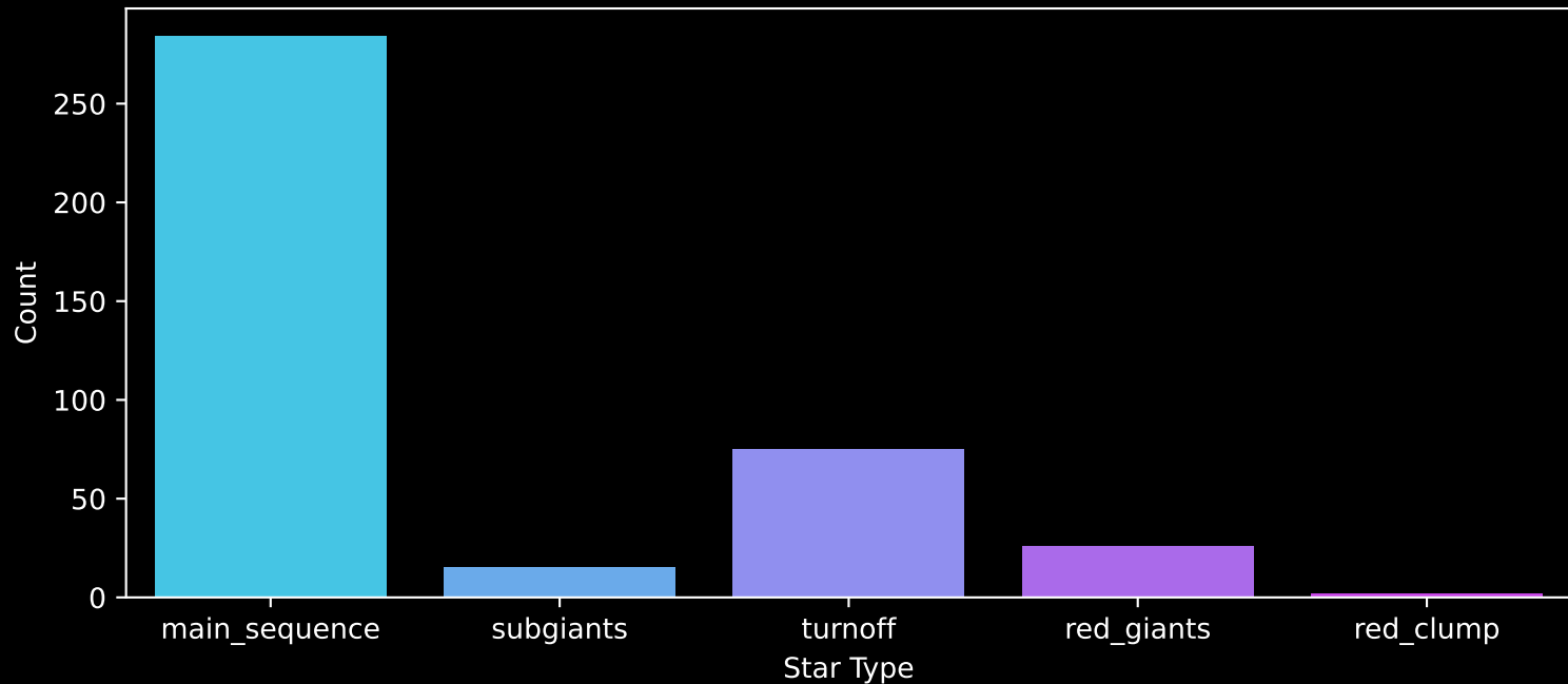
GALAH DR4 Field: [6685] Count plot of Star Type
