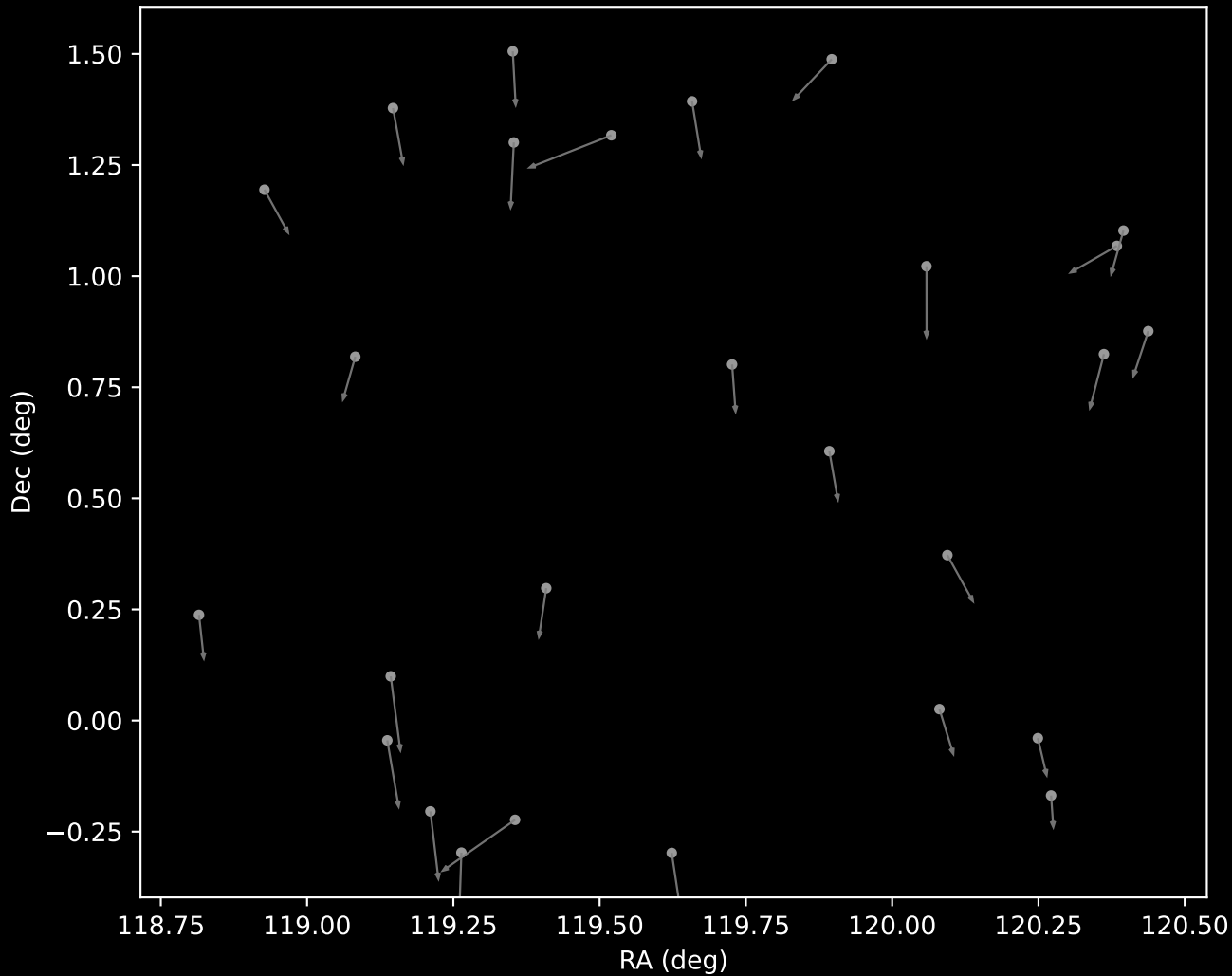
GALAH DR4 Cluster 14 Proper Motion Vectors (n=27)
