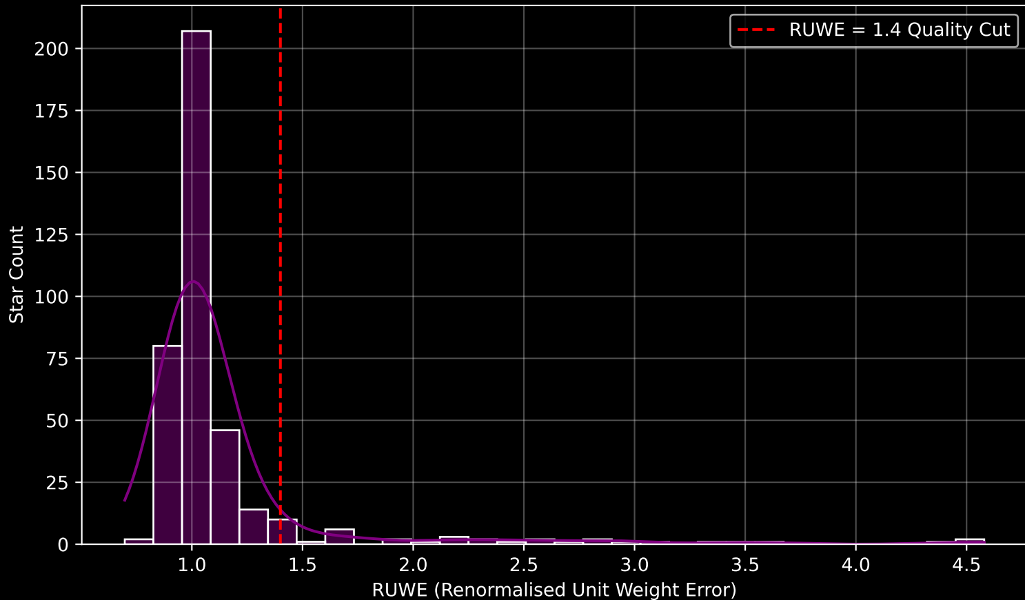
GALAH DR4 Field [6685] RUWE Distribution (n= 388)
