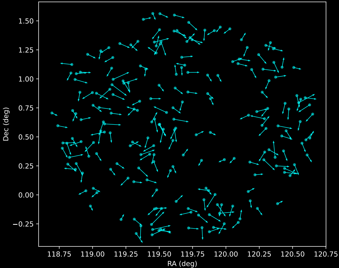
GALAH DR4 Noise Stream Proper Motion Vectors (n=213)
