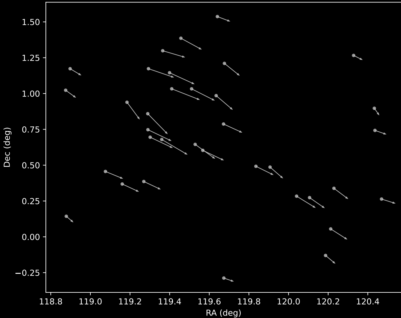
GALAH DR4 Cluster 15 Proper Motion Vectors (n=35)
